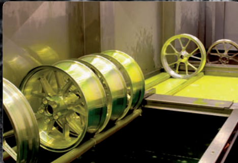
Controllo liquidi penetranti al 100% 100% penetrant liquid testing inspection
