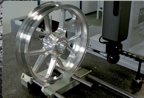
Controllo tridimensionale al 100% 100% 3D tolerance inspection
