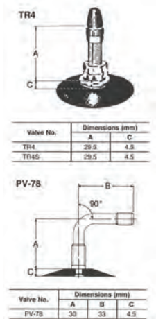
Tube Type Rubber Base Valves
